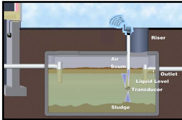
Diagram of 1000 Gallon Grease Trap
